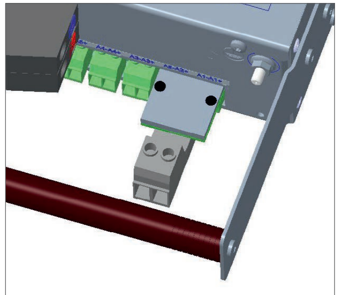
fig. 26: load bridge for the parallel connection of two ESX300-S in plugged-in condition
