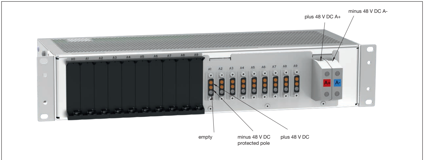
fig.14 version PDB-N-CP09A-FF-Ax, pin assignment
