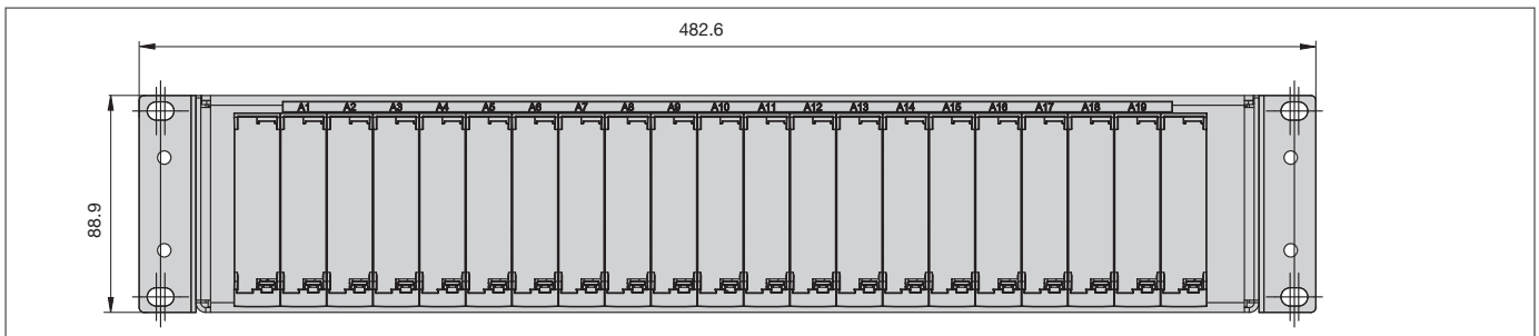
fig. 6: front view PDB-N-CP19A-RR-Ax 1 x 19 slots
