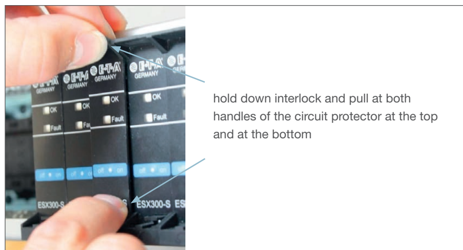
fig. 19: ESX300-S removal
