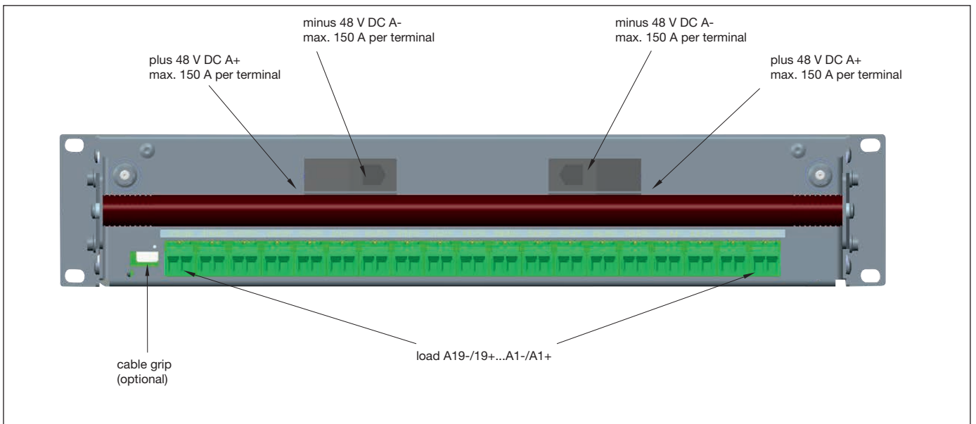
fig. 15: version PDB-N-CP19A-RR-Ax, pin assignment (cable grip installed)
