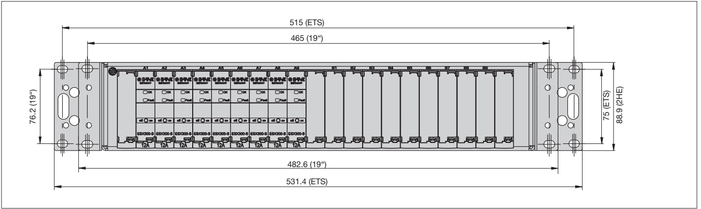
fig. 8: front view PDB-N-CP18R-RR-Ax 2 x 9 slots
