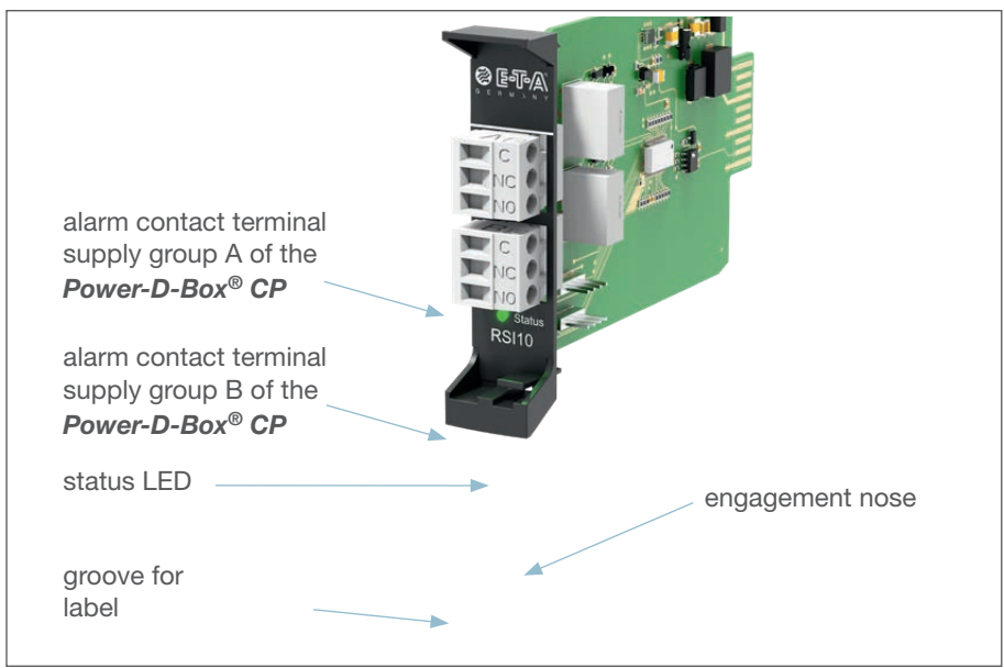
fig. 27: RSI10 sub-assembly
