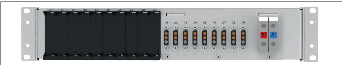
fig. 3: front view PDB-N-CP09A-FF-Ax terminals on the front with high current SUB-D connectors
