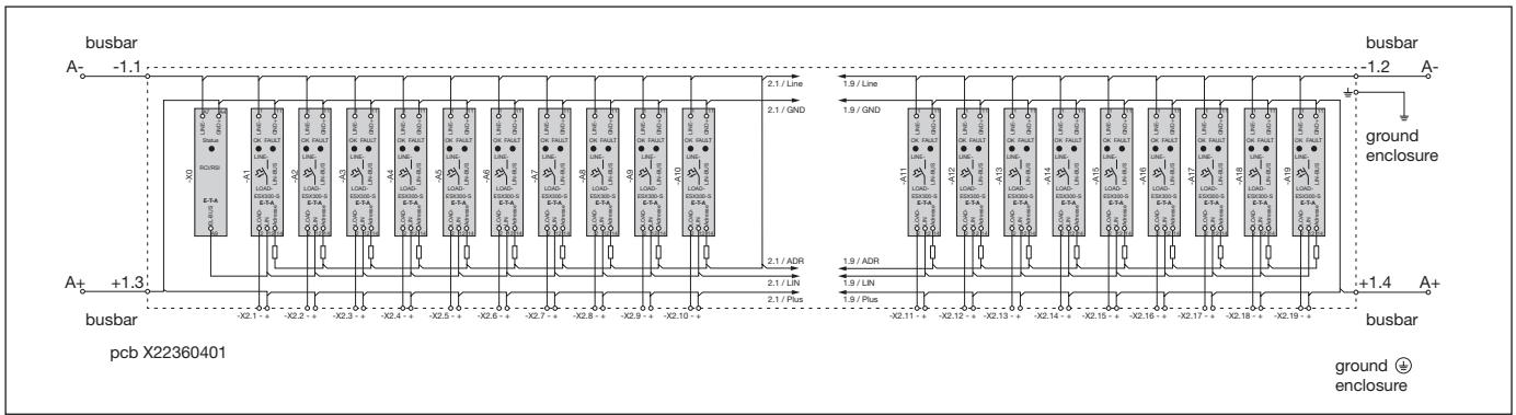
fig. 11: Schematic diagram PDB-N-CP19A-RR-Ax, 1 x 19 slots with signalling
