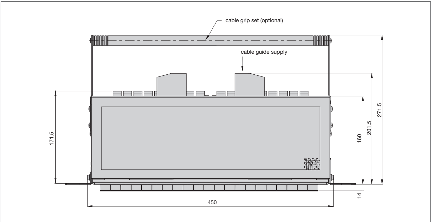
fig. 10: top view PDB-N-CP18R-RR-Ax 2 x 9 slots (with rear cable grip rail)
