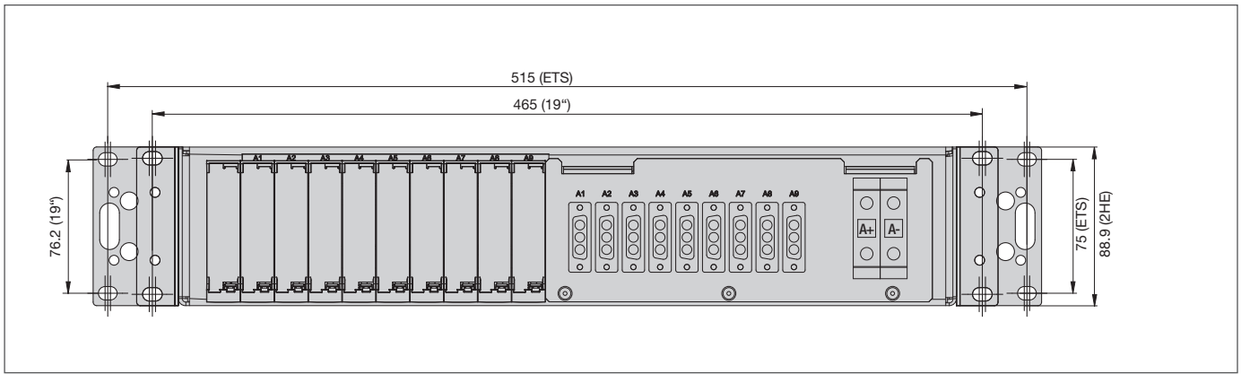
fig. 4: front view PDB-N-CP09A-FF-Ax 1 x 9 slots, terminals on the front with high current SUB-D connectors
