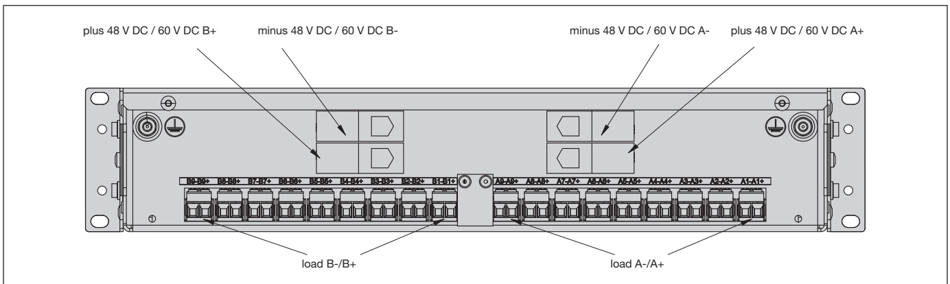
fig. 13: version PDB-N-CP18R-RR-A, pin assignment (cable grip removed)
