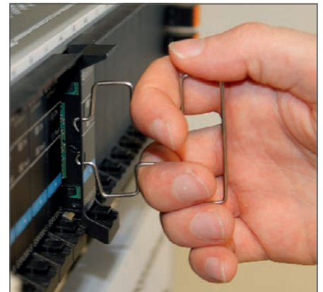
fig. 21: Extracting tool for ESS300-S
