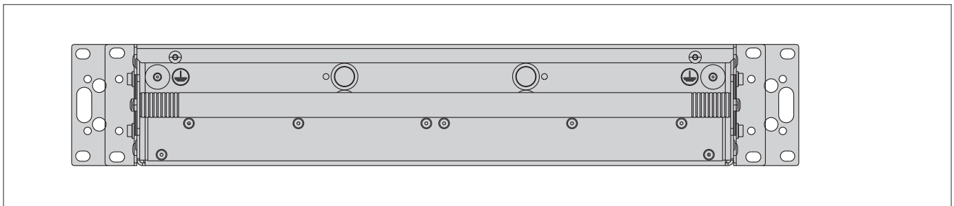
fig. 5: rear view PDB-N-CP09A-FF-Ax 1 x 9 slots (with rear cable grip rail)
