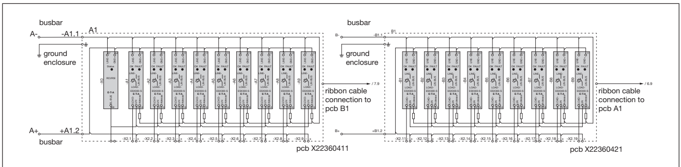
fig. 12: Schematic diagram PDB-N-CP18R-RR-Ax, 2 x 9 slots with signalling
